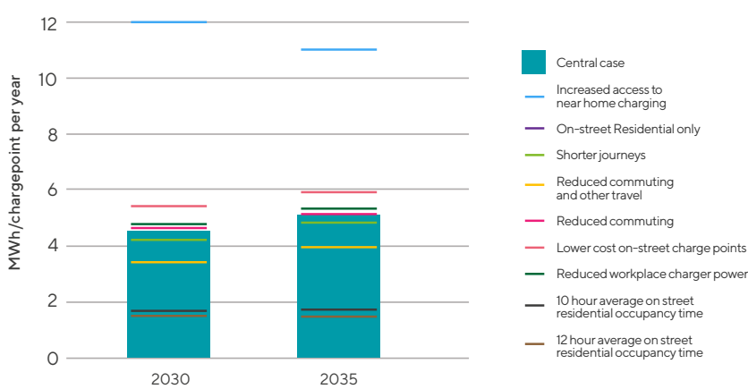
Figure 12 – On-street residential chargepoint throughput (2030 and 2035) and impact of variations to: availability of near home charging; journey lengths; overall vehicle mileage; and upfront costs of on-street residential chargepoints.
