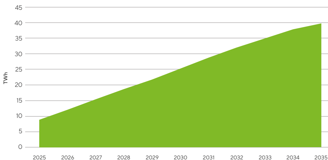
Figure 22 – UK annual electricity demand delivered through home chargepoints (Central case)
