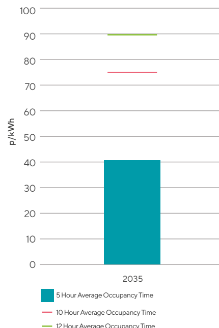
Figure 20 – Prices at on-street residential chargepoints in 2035, for a variety of average occupancy times
